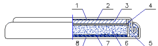
1. Anode cup, 2. Anode collector net, 3. Anode (Lithium metal), 4. Separator, 5. Gasket, 6. Cathode (MnO 2 ), 7. Cathode collector net, 8. Cathode can, Cutaway View of Lithium Manganese Dioxide (Coin type)
